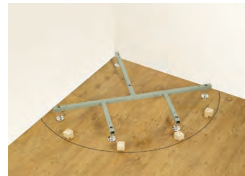
2. Adjustable steel frame for levelling and easy plumbing.
