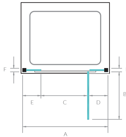
Right Handed Hinged
