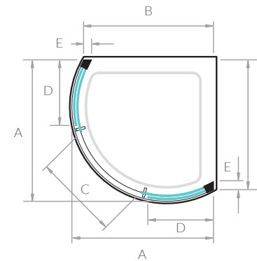
Curved Centre Access
