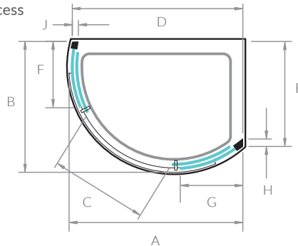
Offset Side Access
