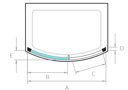
Bowed Sliding Door
