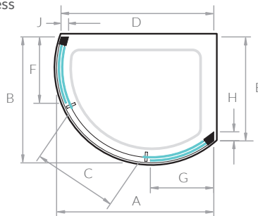
Offset Side Access
