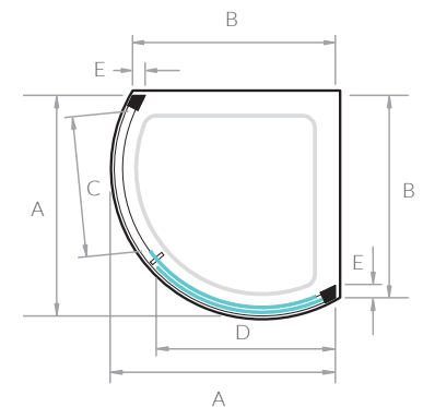
Curved Side Access
