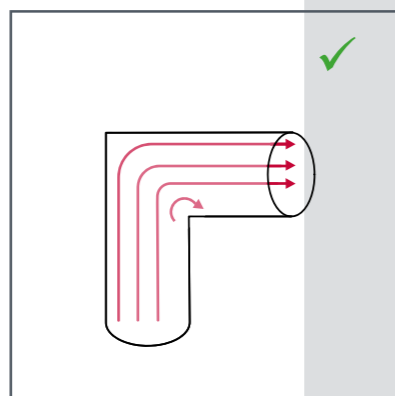
90° square bend. Ok to use, however will increase noise level / decrease air flow.
