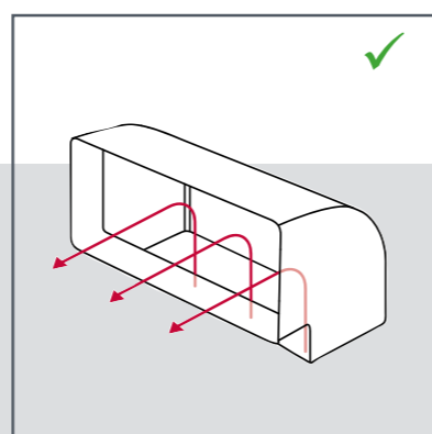
90° bend. Recommended.
